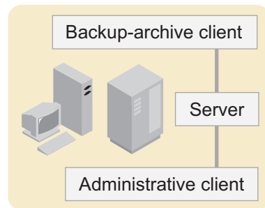
Figure 65. Stand-alone environment
