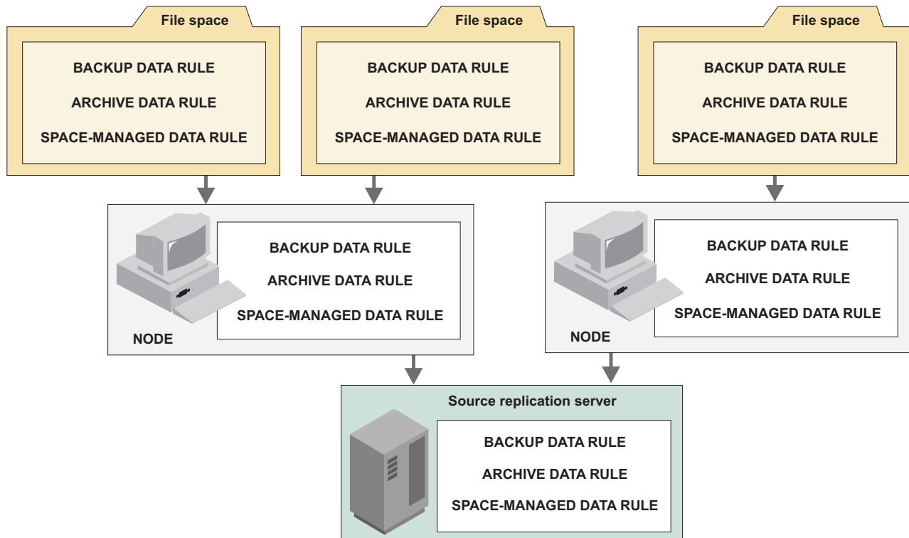
Figure 111. Replication-rule hierarchy
