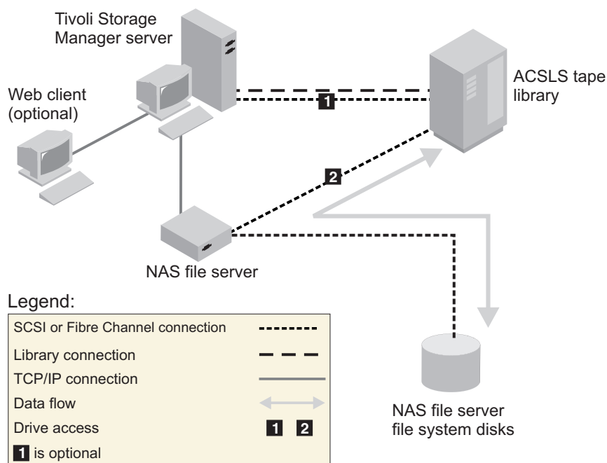
Figure 19. Configuration 4: ACSLS library connected to the Tivoli Storage Manager server
